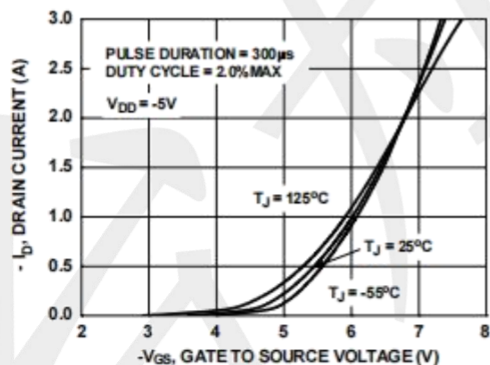
Figure 5. Transfer Characteristics
