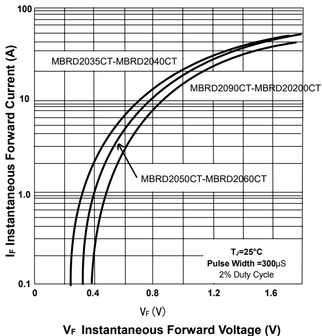
FIG1-TYPICAL FORWARD CHARACTERISTIC
