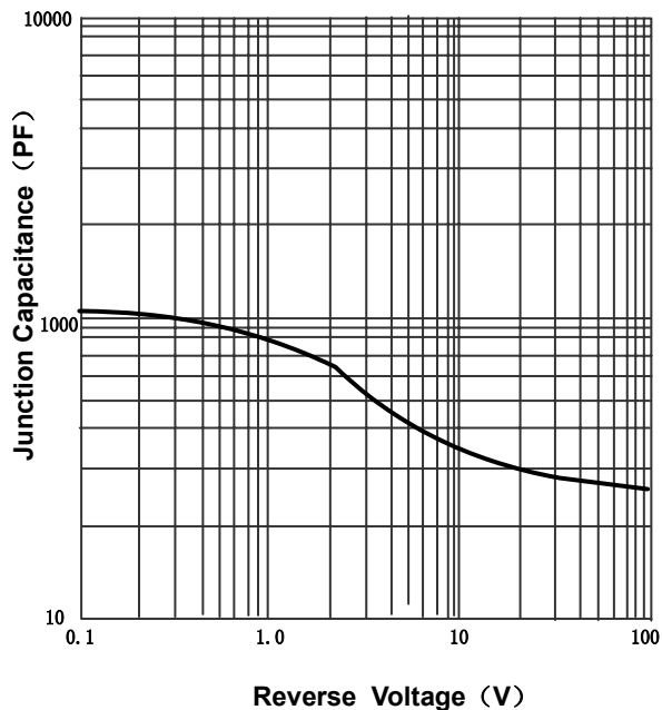
FIG4-TYPICAL RECERSE CHARACTERISTICS
