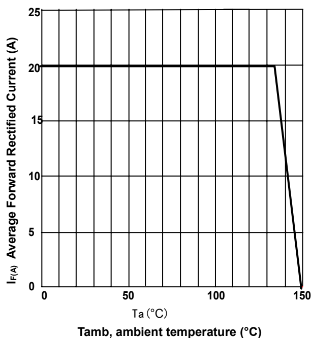
FIG2-FORWARD CURRENT DERATING CURVE
