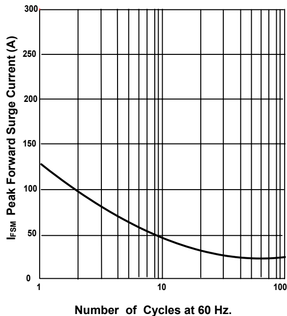
FIG3-MAXIMUM NON REPETITIVE PEAK FORWARD SURGE CURRENT
