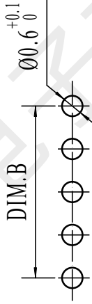
PCB LAYOUT
