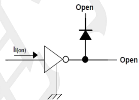
Fig.4 I_i Test Circuit
