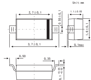
SOD-123
