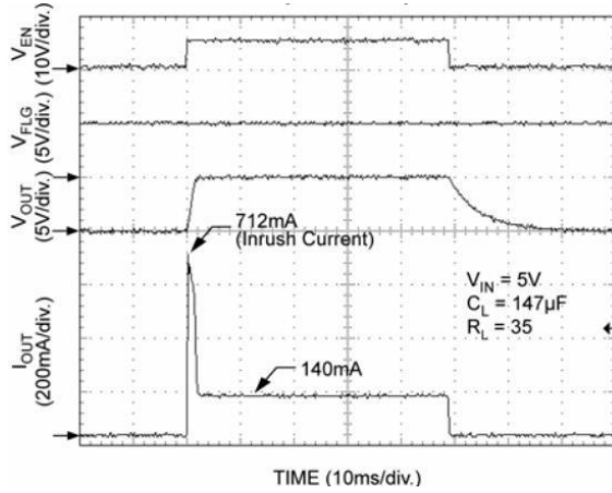
Turn-On/Turn-Off (XL2026-1)
