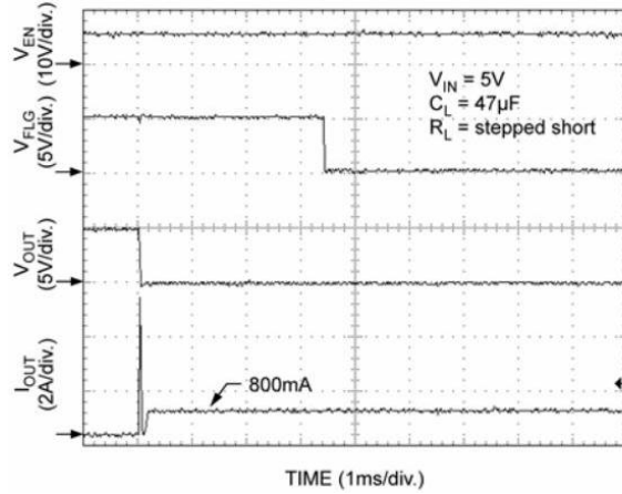
Current-Limit Response (Stepped Short-XL2026-1)
