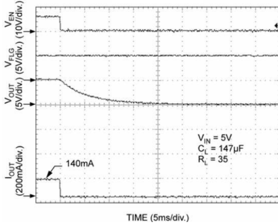
Turn-Off (XL2026-1)
