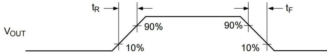
Output Rise and Fall Times
