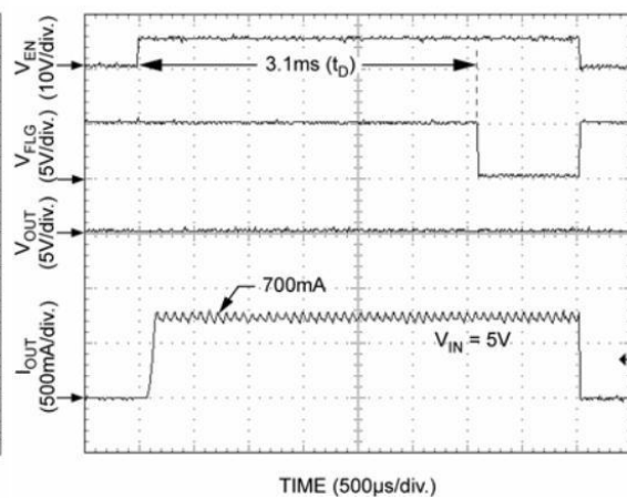
Enabled Into Short (XL2026-1)
