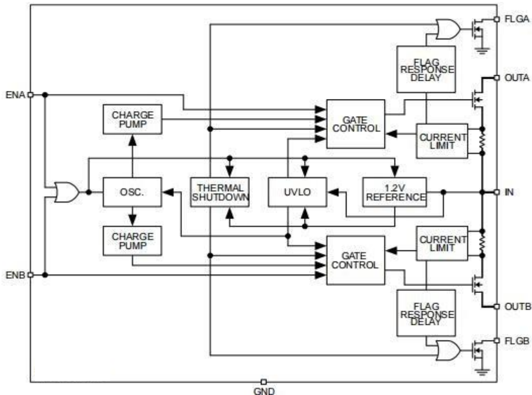
XL2026 Block Diagram
