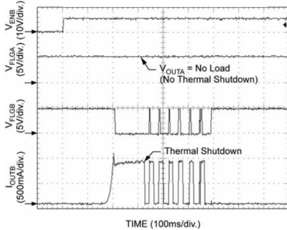
Independent Thermal Shutdown (XL2026-1)
