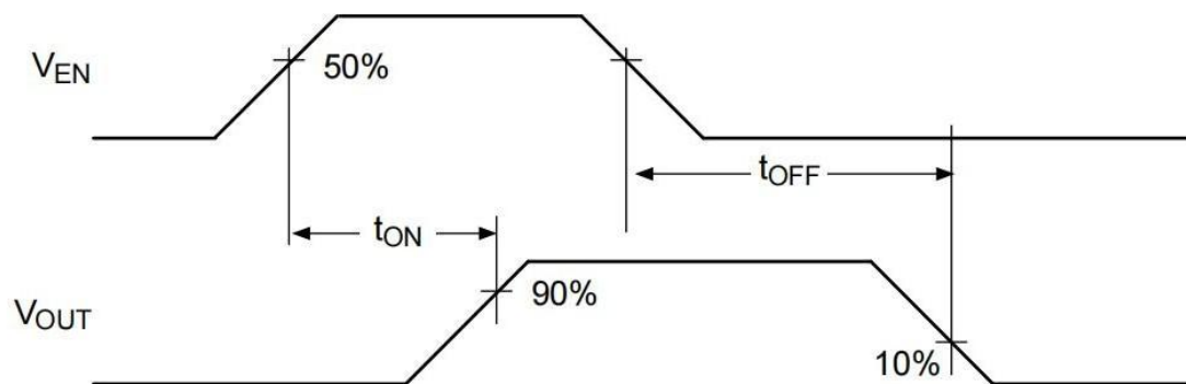
Active-High Switch Delay Time (XL2026-1)
