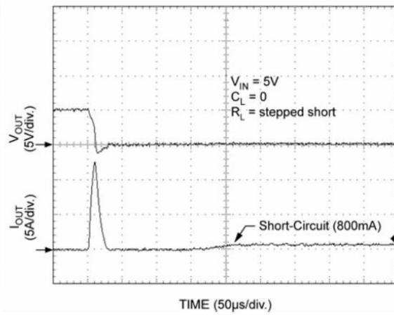
Current-Limit Response (XL2026-1)
