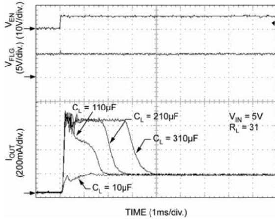
Inrush Current Response (XL2026-1)
