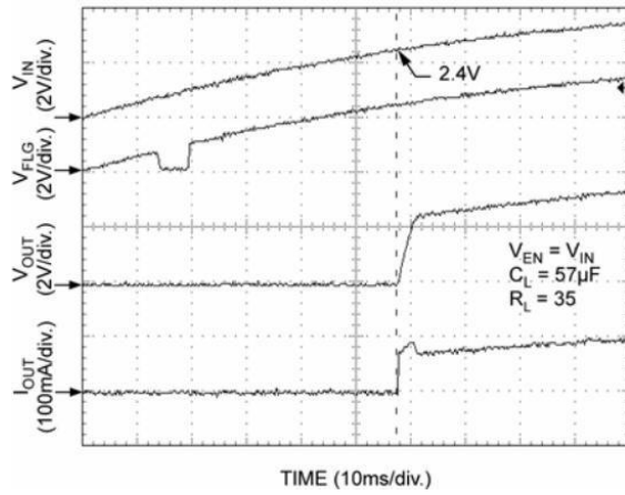
UVLO- V_{IN} Rising (XL2026-1)
