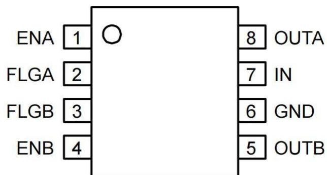
8-Pin SOP
