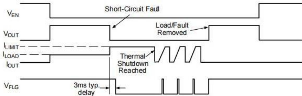
Figure 1. XL2026-2 Fault Timing
