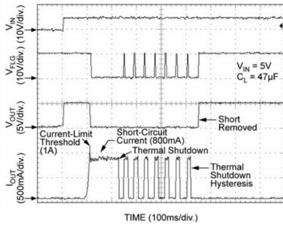
Current-Limit Response (Ramped Load-XL2026-1)
