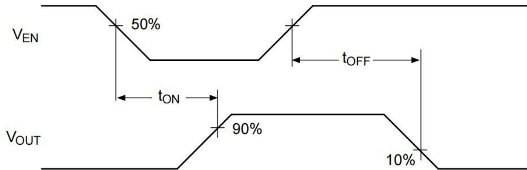
Active-Low Switch Delay Times(XL2026-2)
