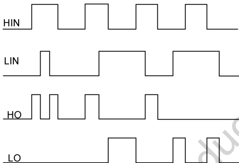
Figure 5. IRS2807DS Input and output timing waveform
