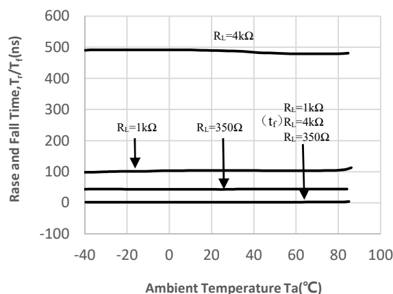
Fig.8 Rise and Fall Time vs. Ambient Temperature
