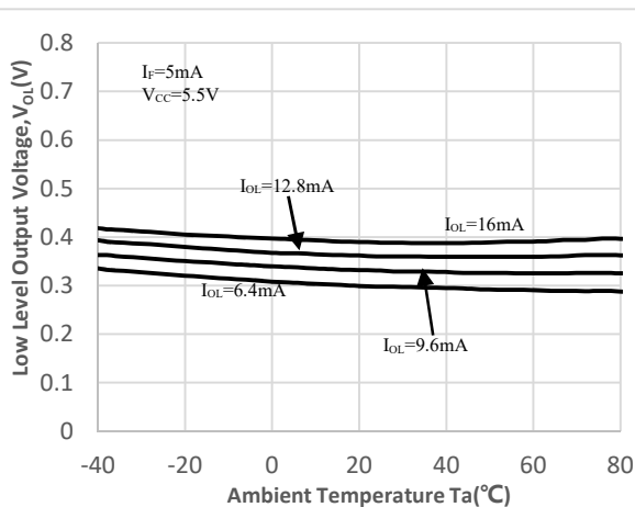
Fig.2 Low Level Output Voltage vs. Ambient Temperature
