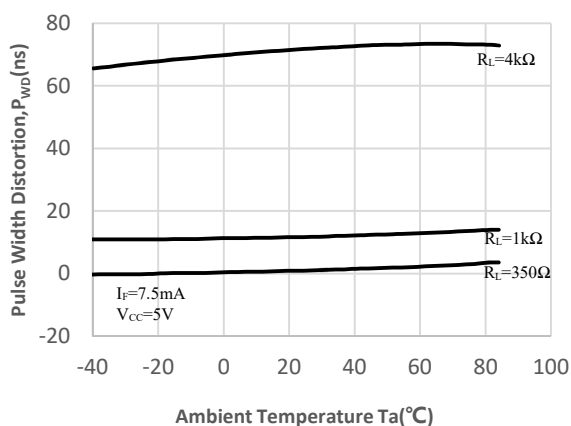
Fig.7 Pulse Width Distortion vs. Ambient Temperature
