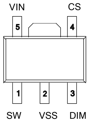
SOT89-5
