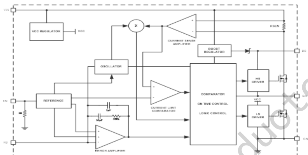
Figure 2. AOZ1282CI Block Diagram
