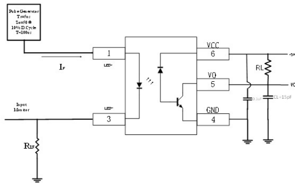
Fig.7 Test Circuit and Waveforms for t_{PLH} , t_{PHL} , t_r and t_f
