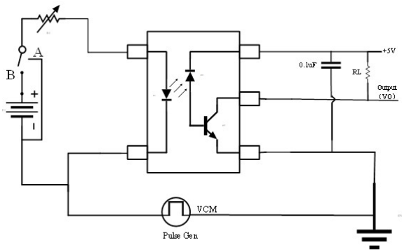
Fig.8 Test Circuit Common Mode Transient Immunity
