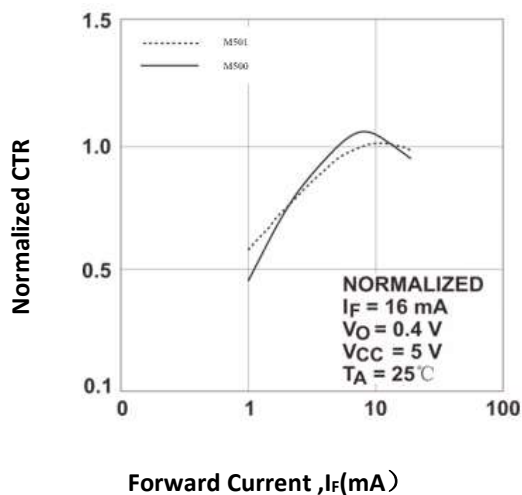
Fig.1 Normalized CTR vs Forward Current
