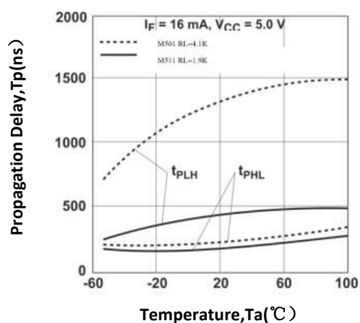
Fig. 5 Propagation Delay vs Temperature
