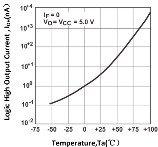
Fig.4 Logic High Output Current vs Temperature
