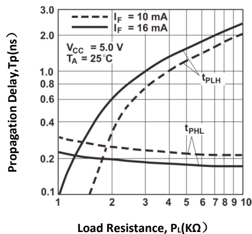
Fig.6 Propagation Delay vs Load Resistance
