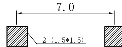
PCB LAND PATTERN
