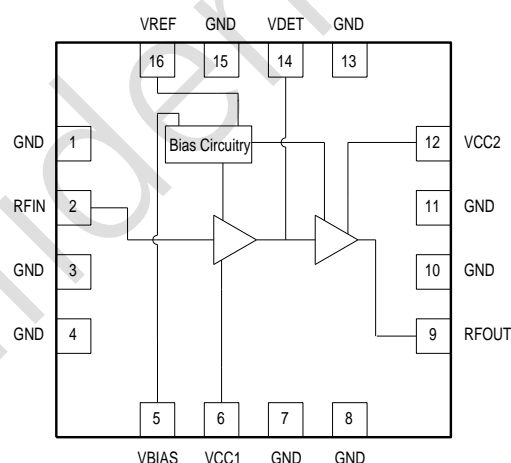
Figure 2. GSM2424 Function Block Diagram
