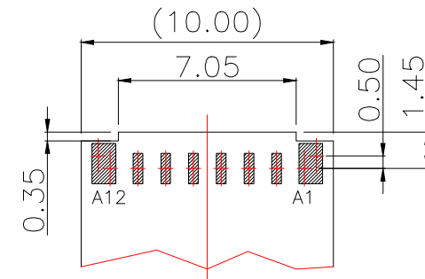
RECOMMENDED PCB LAYOUT(TOP VIEW) THICKNESS SEE TABLE1;DEFAULT TOLERANCE:±0.05
