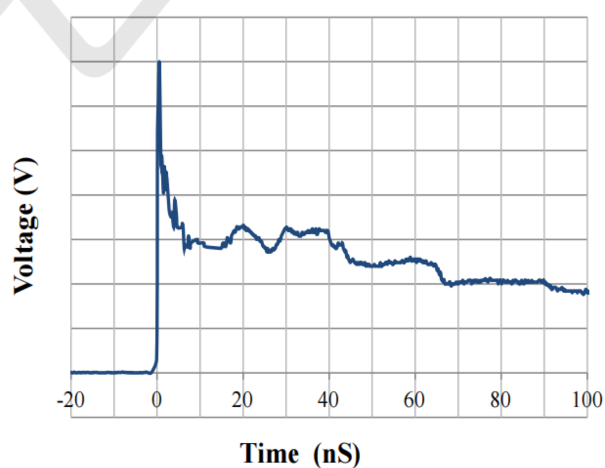
IEC61000-4-2 Pulse Waveform
