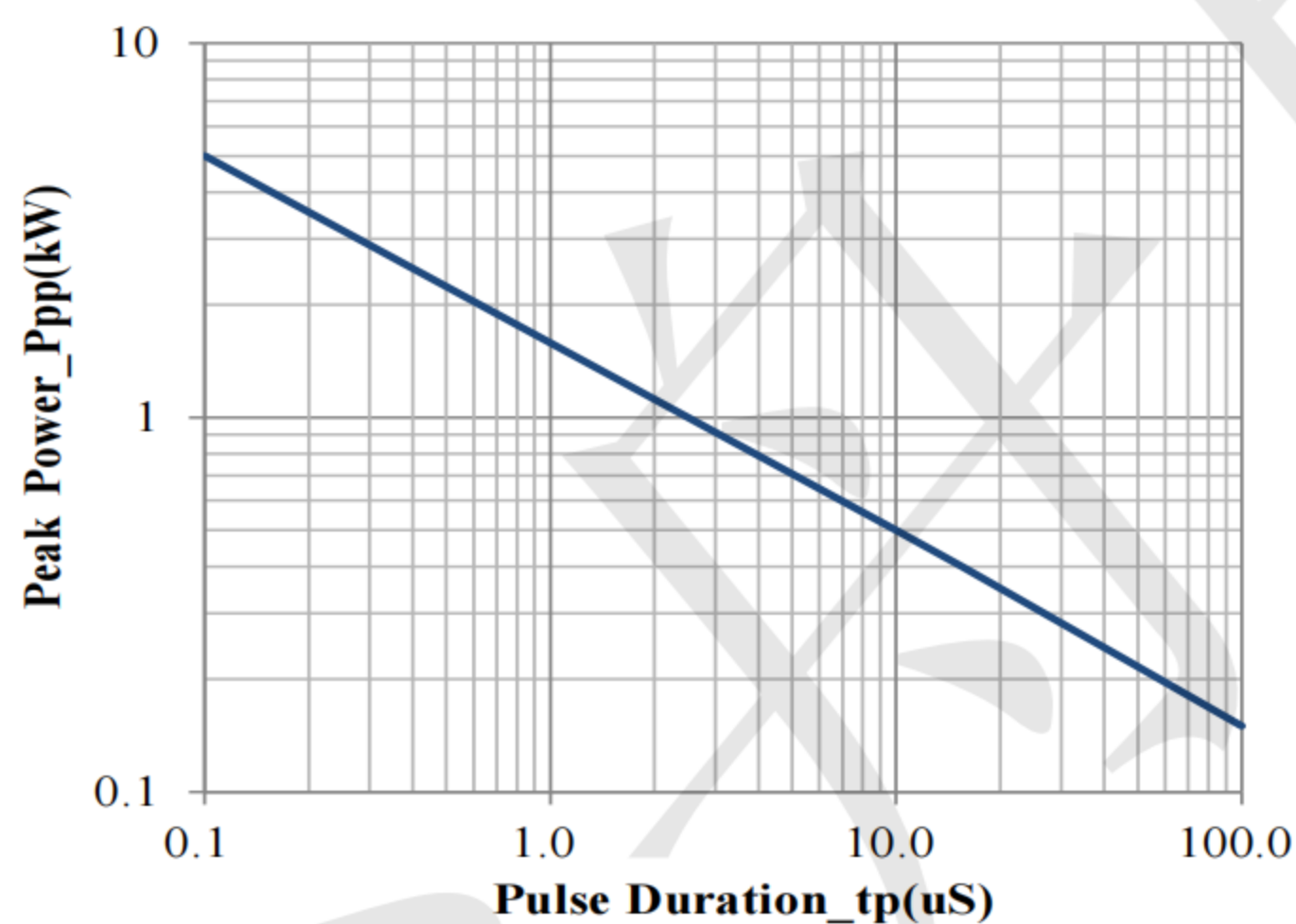
Peak Pulse Power vs. Pulse Time
