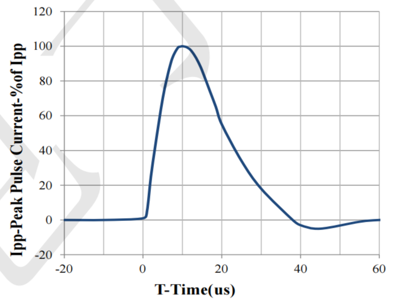
8 X 20us Pulse Waveform
