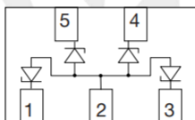
DFN1308-5 (Top View)
