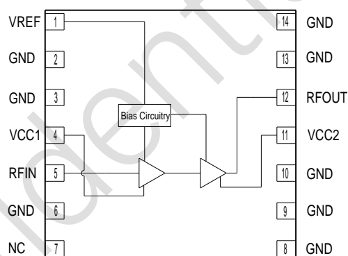
Figure 2. GSM2124C Function Block Diagram
