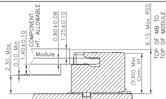
Assembly stack height schematic diagram
