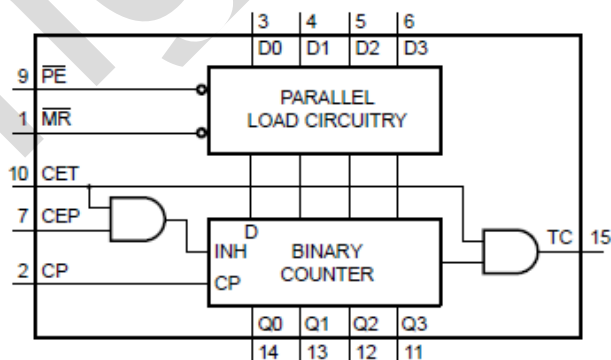
Figure 3. Functional diagram
