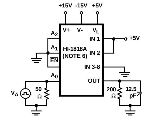
FIGURE 2B. TEST CIRCUIT
