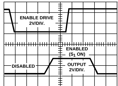
FIGURE 1C. WAVEFORMS
