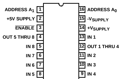
HI-1828A (CERDIP) TOP VIEW
