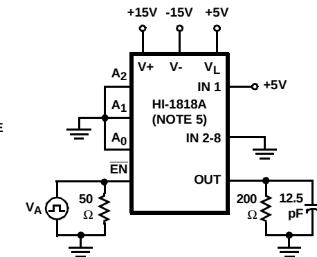
FIGURE 1B. TEST CIRCUIT
