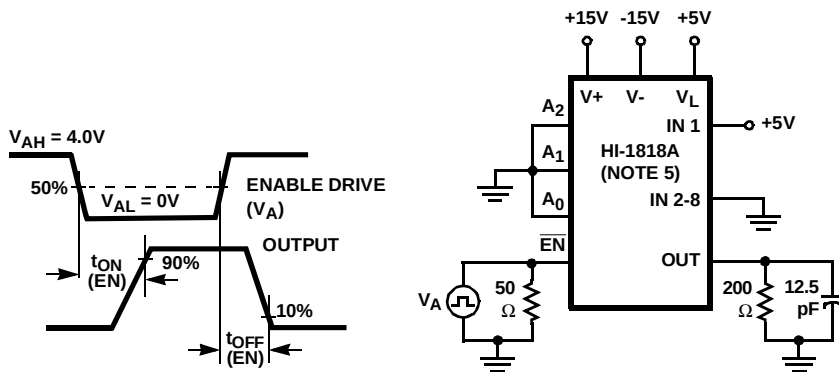
FIGURE 1A. MEASUREMENT POINTS
