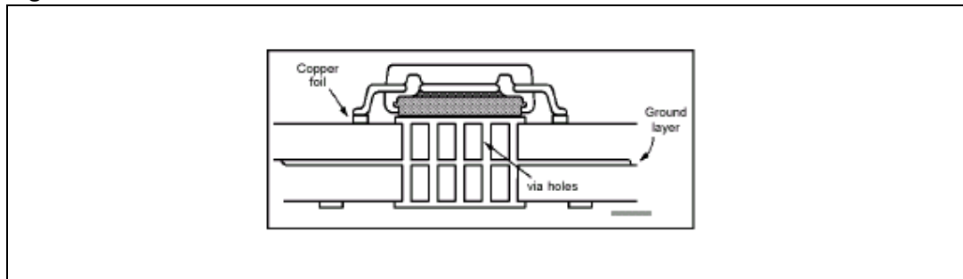
Figure 7. Thermal characteristic
