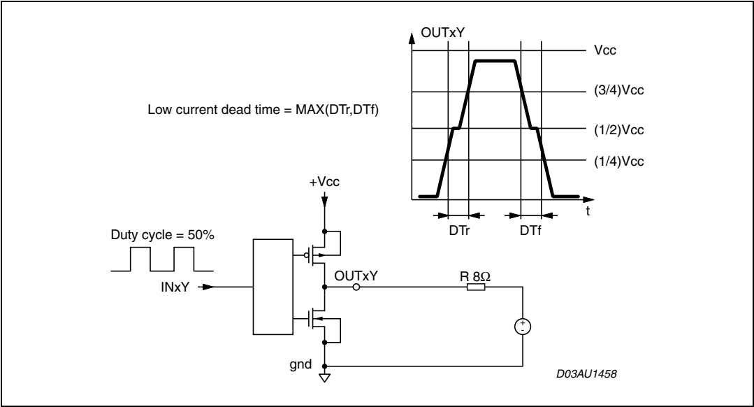
Figure 3. Resistive load
