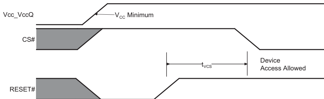
Figure 20. Power-up with RESET# LOW
