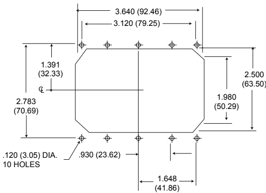
Rear Mount
