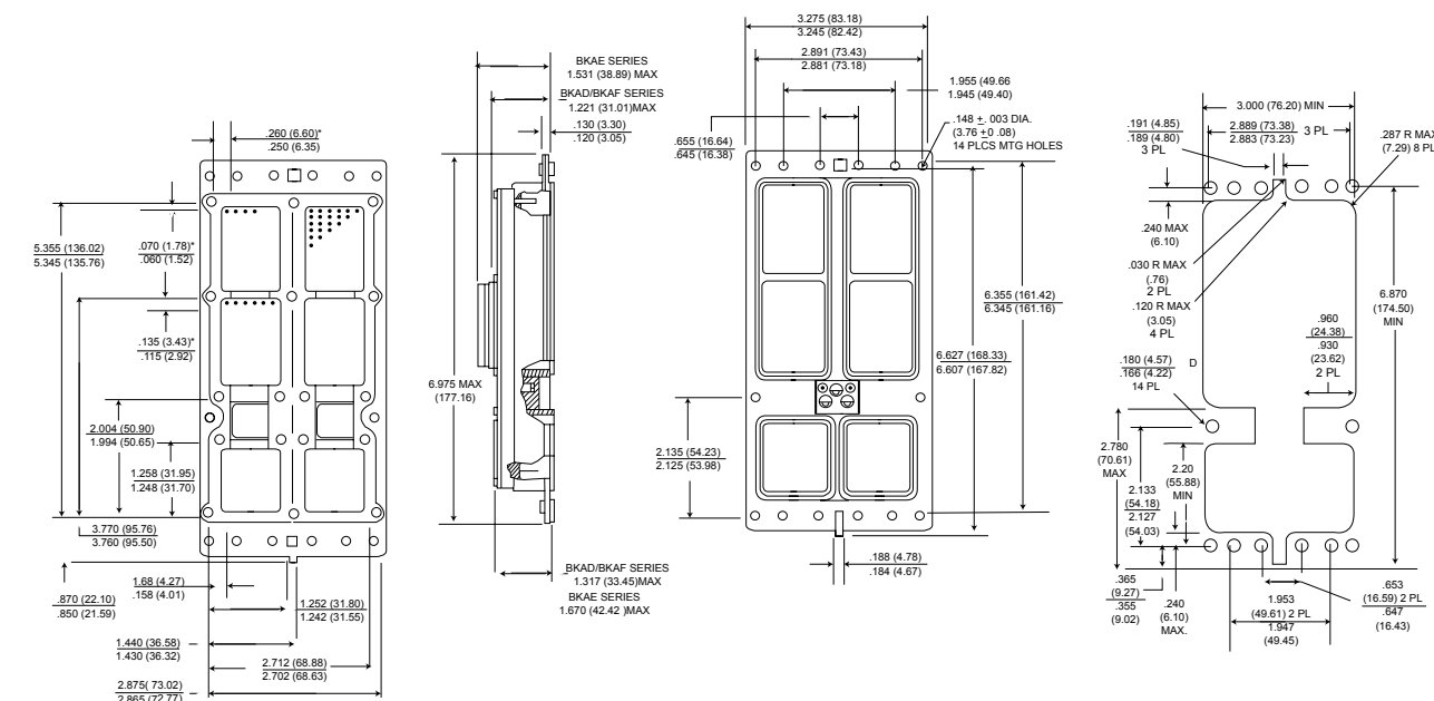
Retainer Plate
