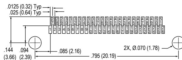
51 Contacts
