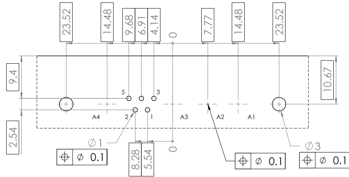
PCB hole pattern, mounting side
