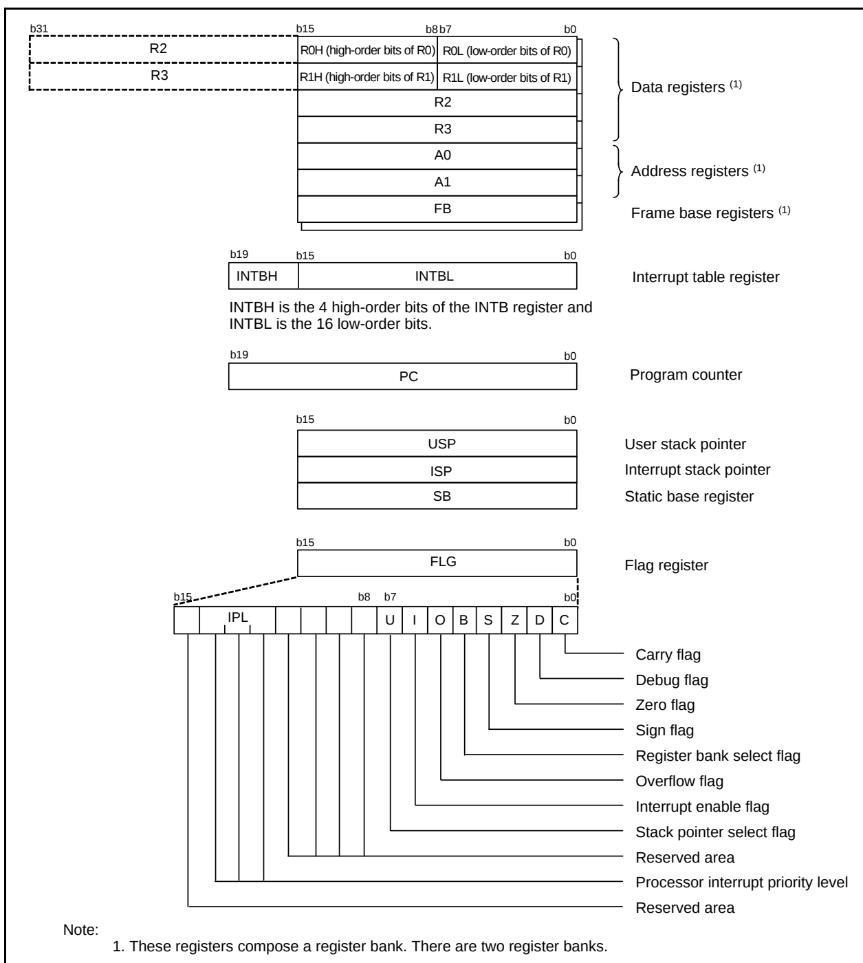
Figure 2.1 CPU Registers
