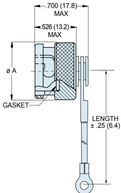
Receptacle Cover 660-083
