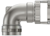
Spin Coupling
