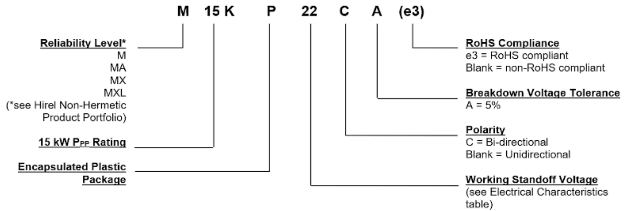
Figure 2-1. Part Nomenclature
