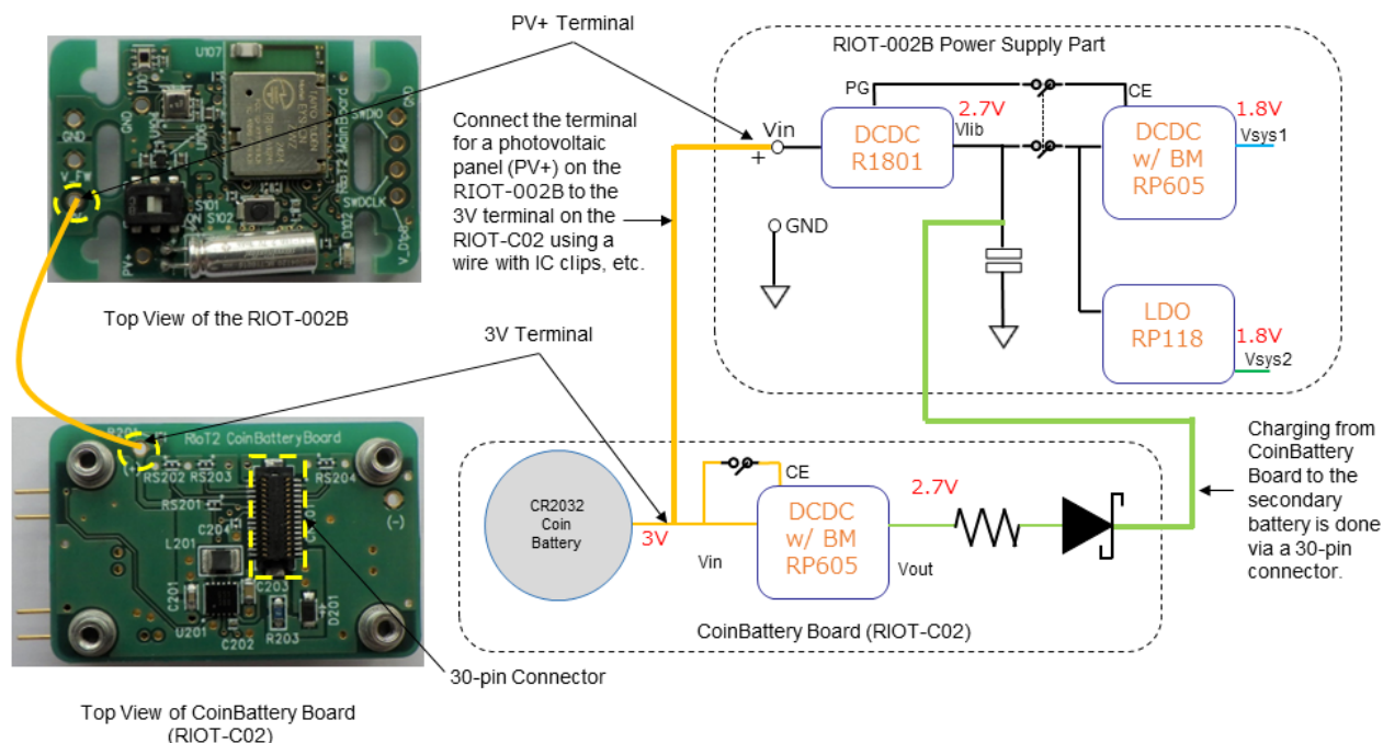
Figure 3. Connection between 3V Terminal of Coin Battery Board and PV+ Terminal of RIOT-002B
