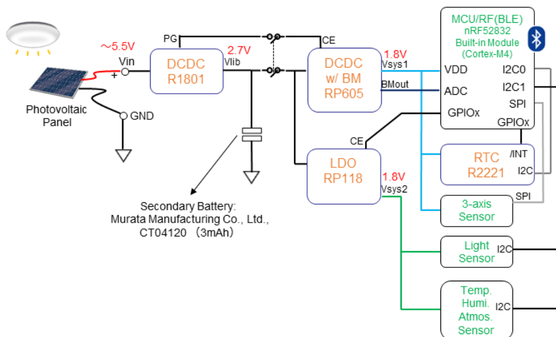
Figure 2. Block Diagram of RIOT-002B
