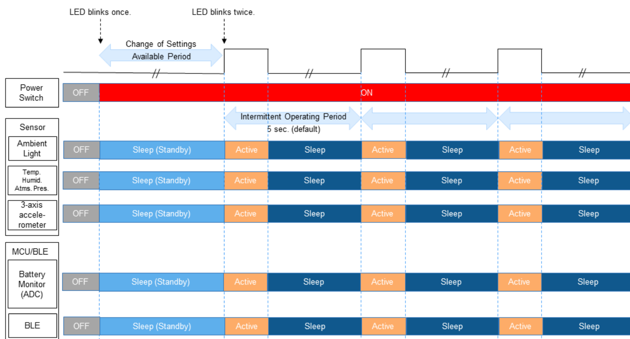
Figure 4. Diagram of Intermittent Operation with Default Firmware
