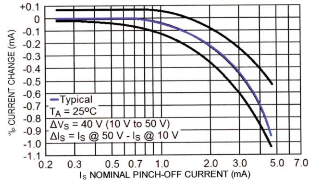
FIGURE 4 – CURRENT REGULATION FACTOR
