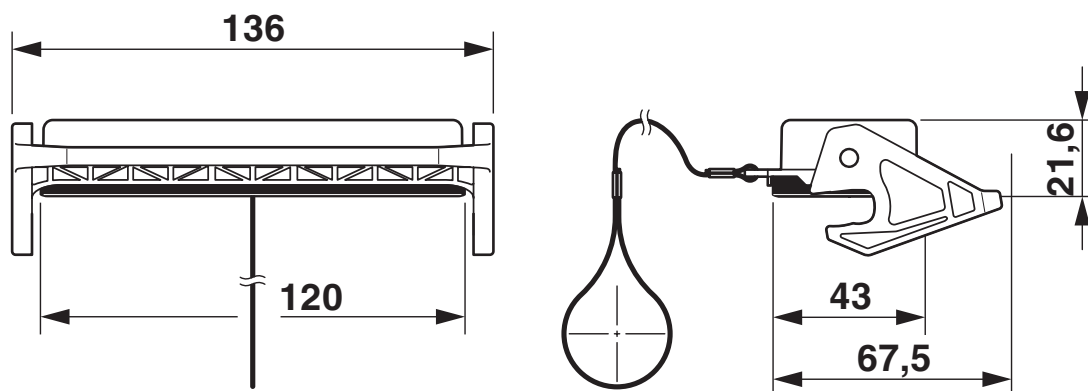
Dimensional drawing
