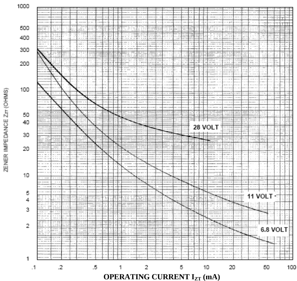
FIGURE 3 ZENER IMPEDANCE VS. OPERATION CURRENT
