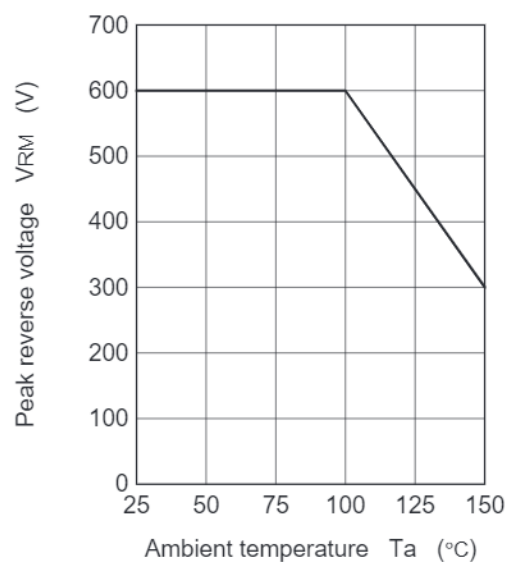
Fig.7 Peak reverse voltage vs. Ambient temperature
