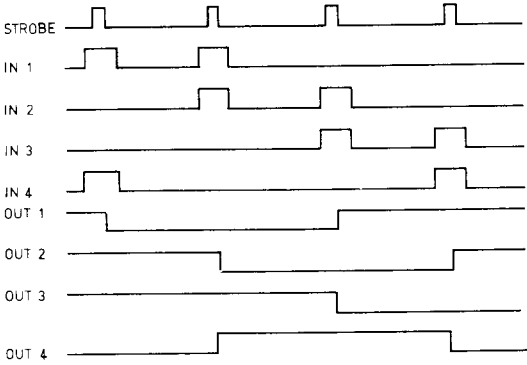
UNIPOLAR 2-PHASE DRIVE
