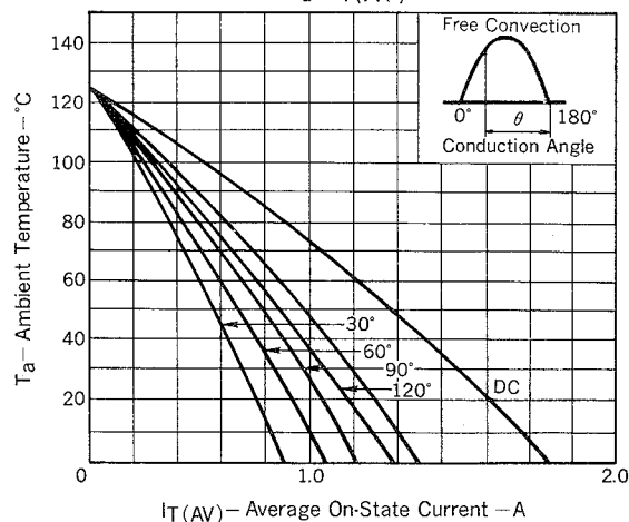
Fig. 6 T_a-I_{T(AV)} RATING
