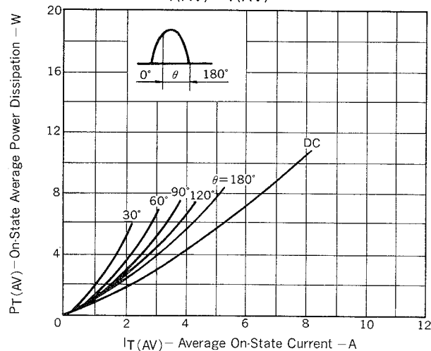
Fig. 4 P_{T(AV)}-I_{T(AV)} CHARACTERISTIC
