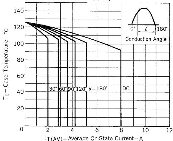
Fig. 5 T_c-I_{T(AV)} RATING
