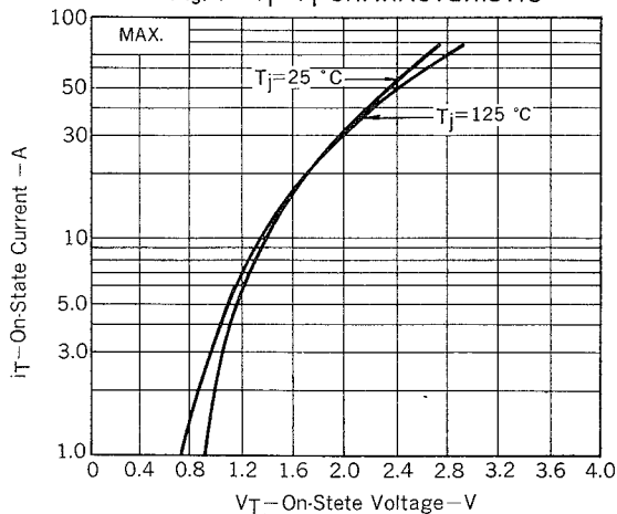
Fig. 1 i_T-v_T CHARACTERISTIC
