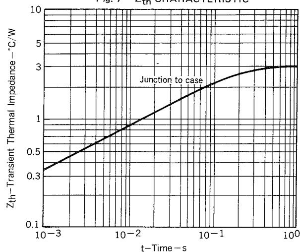
Fig. 7 Z_{th} CHARACTERISTIC
