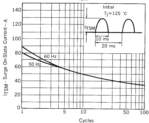
Fig. 2 I_{TSM} RATING
