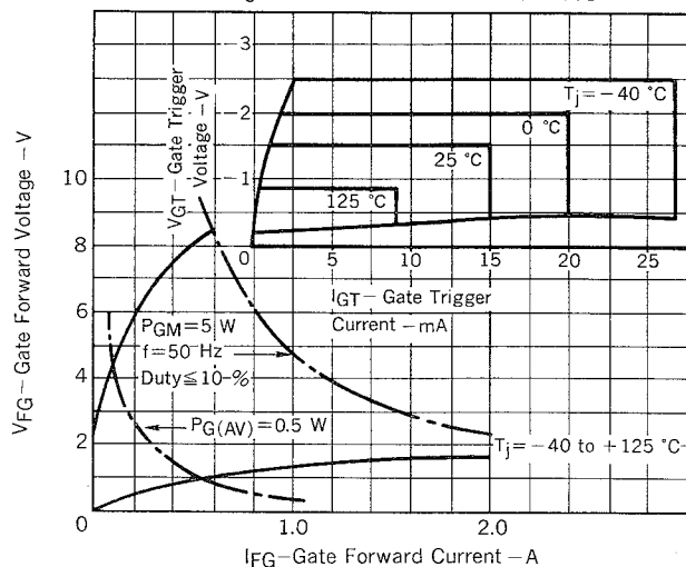
Fig. 3 GATE CHARACTERISTIC
