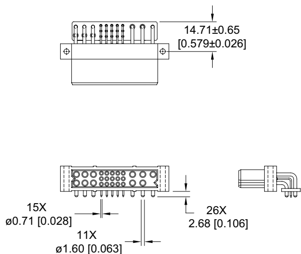
CONNECTOR DIMENSIONS
