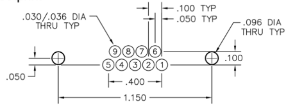
PLUG PC BOARD LAYOUT COMPONENT SIDE
