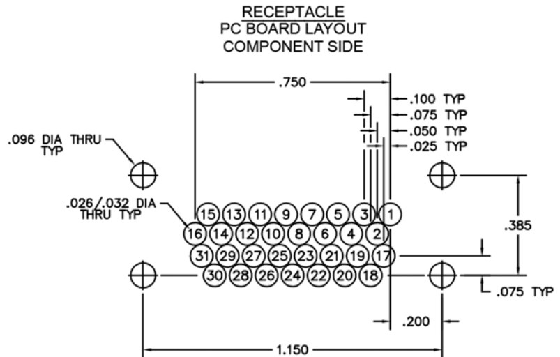
PC BOARD LAYOUT COMPONENT SIDE
