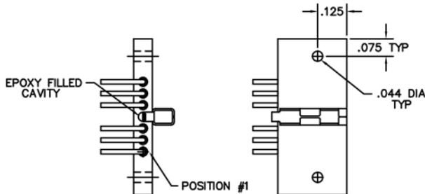
TERMINATION VIEW
