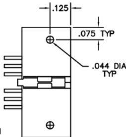
PLUG
