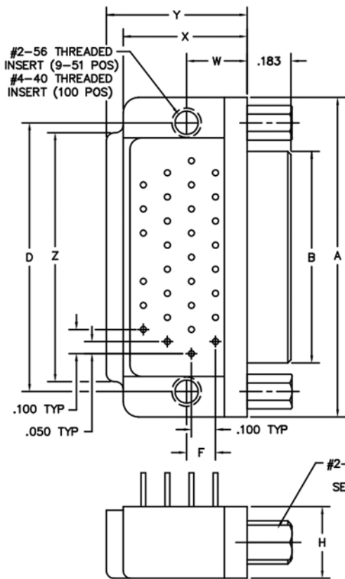
PLUG
