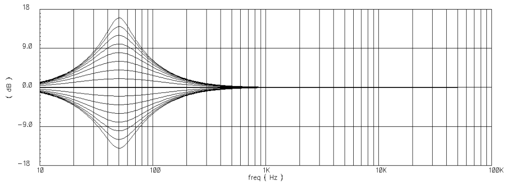
Gain control : +16dB to -14dB/2dB step ( f_0=50\text{Hz} , Q=1.0 )
