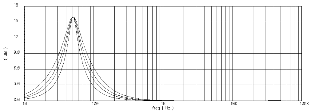
Quality factor : 1.0 / 1.25 / 1.5 / 2.0 ( G_v=+16\text{dB} , f_0=50\text{Hz} )
