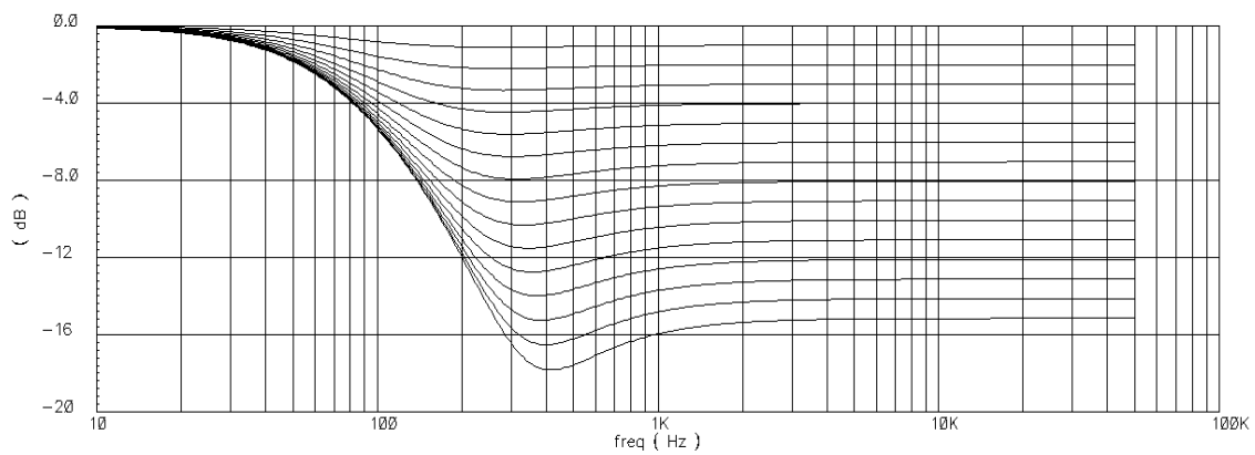
Gain control : 0dB to -15dB/1dB step (f0=400Hz)
