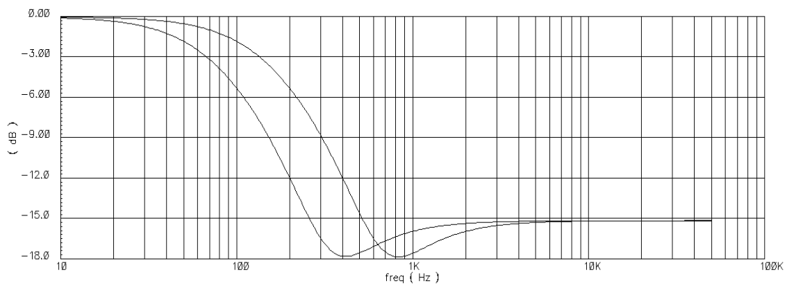
Center frequency : 400Hz / 800Hz (Gv=-15dB)
