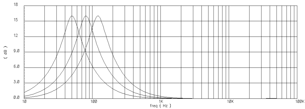
Center frequency : 50Hz / 80Hz / 120Hz ( G_v=+16\text{dB} , Q=1.0 )
