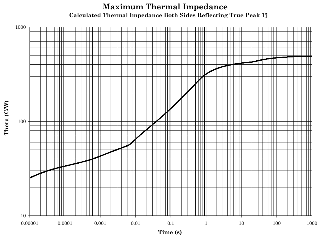
FIGURE 6. Both sides: Thermal resistance = 500°C/W, Pt = 350 mW.
