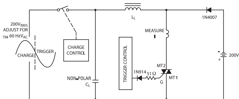
Figure 16. Simplified Test Circuit to Measure the Critical Rate of Rise of Commutating Current (di/dt)
