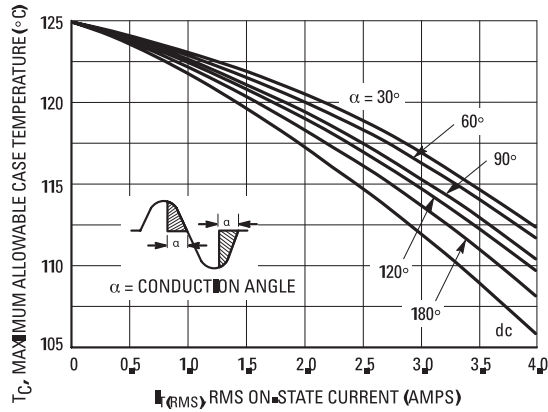
Figure 1. Typical RMS Current Derating
