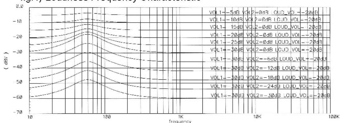
fig.2) Loudness Frequency Characteristic(VOL=-30dB,Loudness=20dB,fO=Variable)
