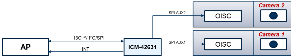
Figure 7. ICM-42631 System Block Diagram
