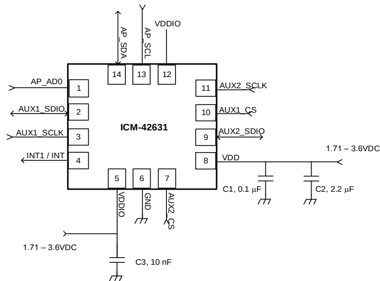
Figure 5. ICM-42631 Application Schematic (I3C SM / I 2 C Interface to Host & SPI-3 Interface for AUX1 & AUX2)
