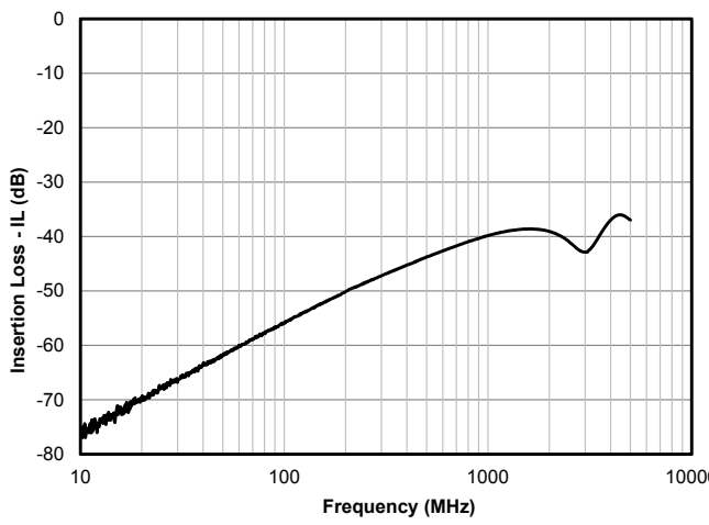
Analog Crosstalk
