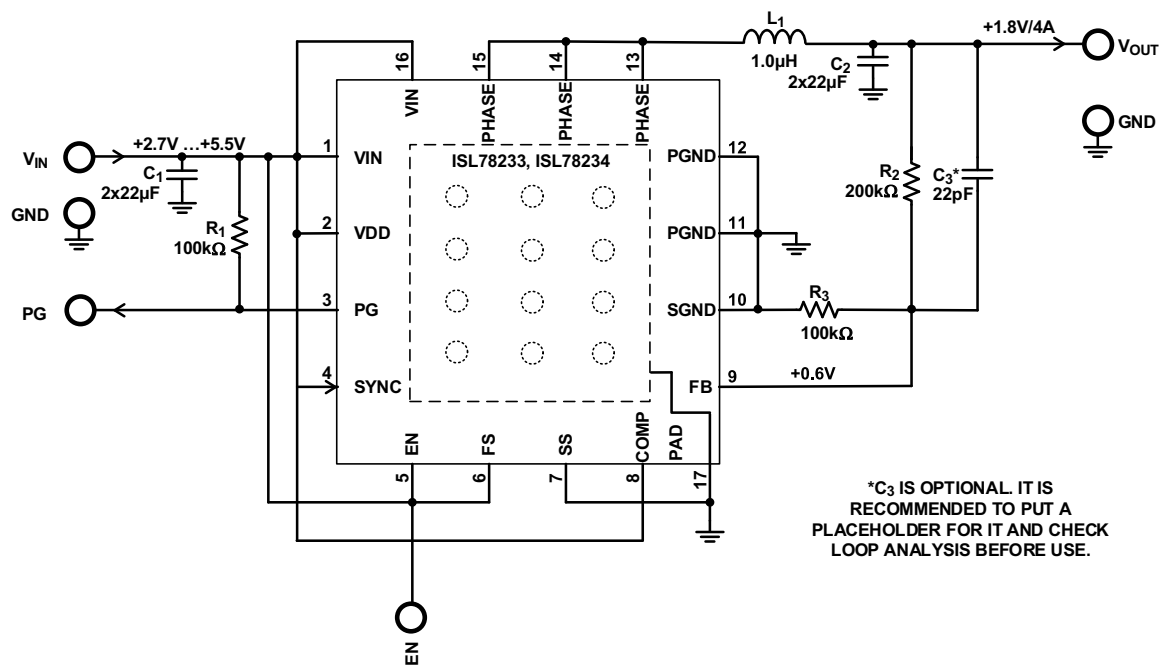
FIGURE 2. TYPICAL APPLICATION DIAGRAM
