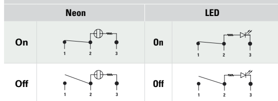
Circuit Diagram
