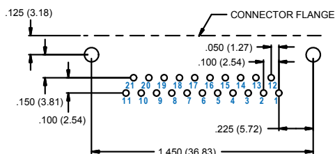
21 PIN M83513/16-C
