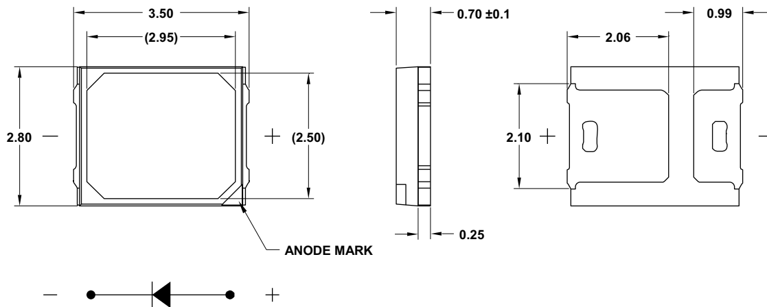
Figure 1: Package Drawing
