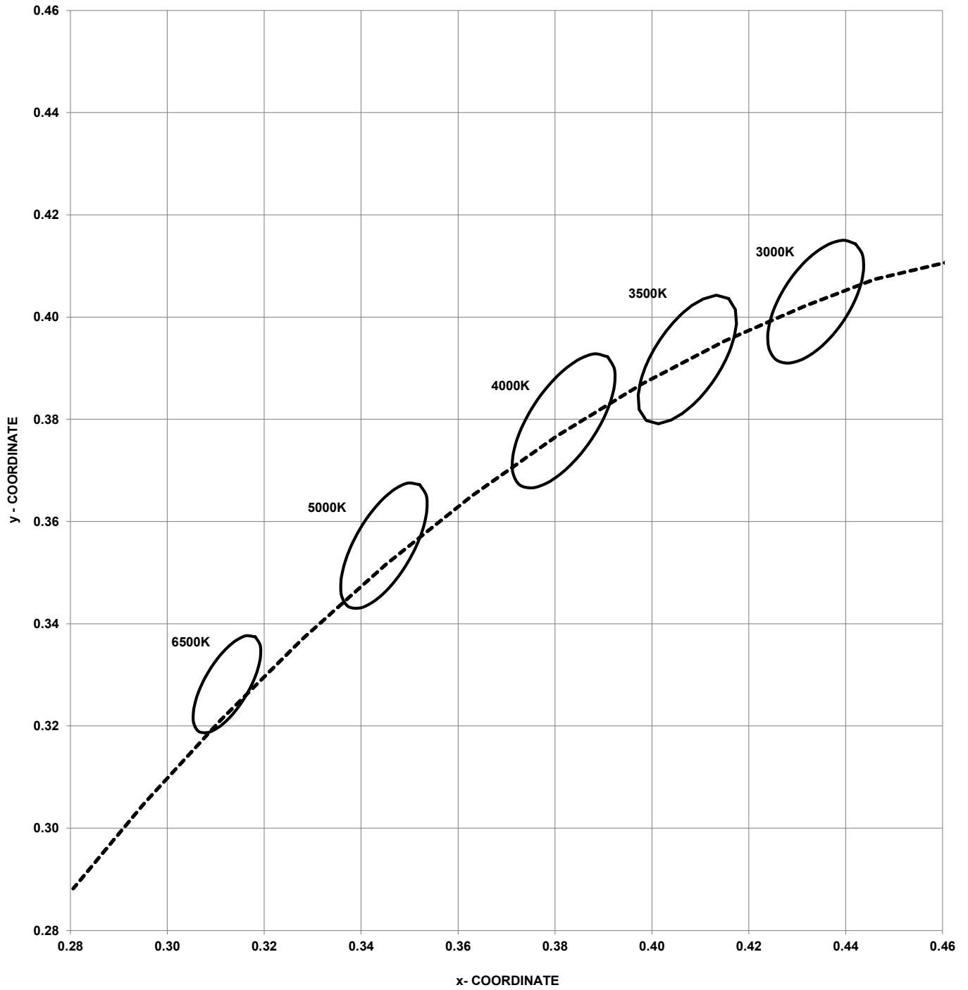
Figure 3: Chromaticity Diagram
