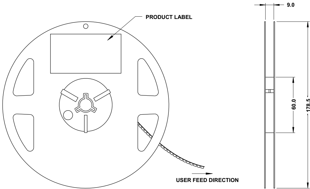
Figure 22: Reel Dimensions
