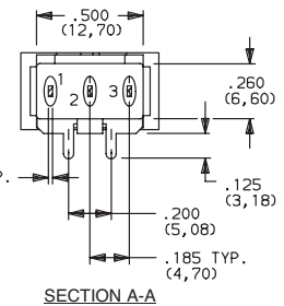
PC MOUNTING
